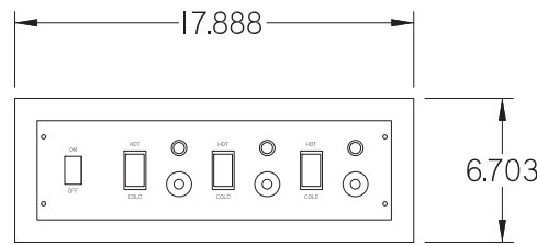
CONTROL PANEL
